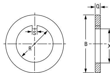
Fig. 54. Tongued washers.
