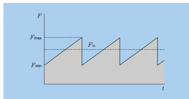
Fig. 4.10 Linear fluctuating load
