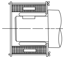
Inner Ring removal using Induction Heater
