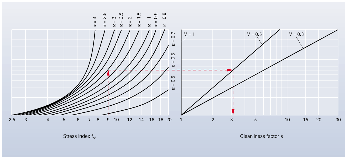
11: Diagram for the determination of cleanliness factor s
