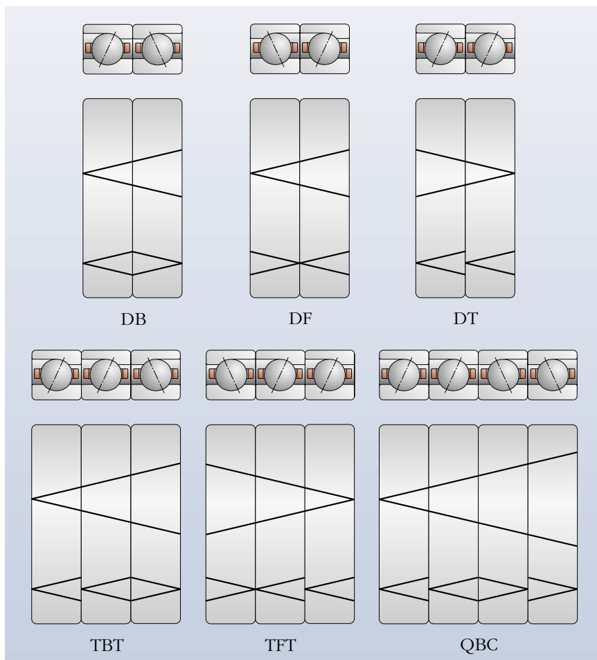
Examples of ready-to-mount bearing sets
