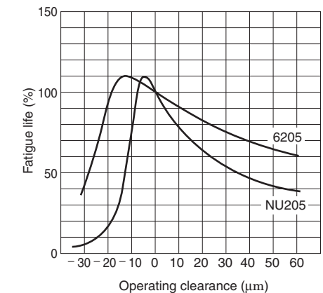
Fig. 10-2 Relationship between operating clearance and fatigue life
