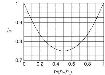
Fig. 5-12 Coefficient f_m
